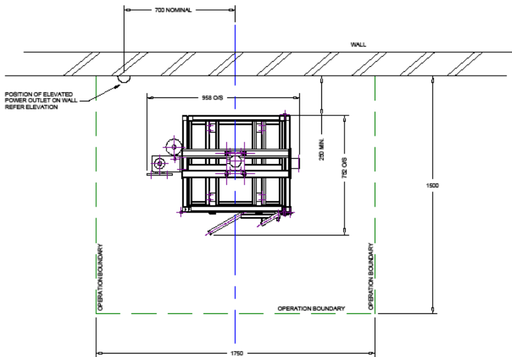
PLAN VIEW
